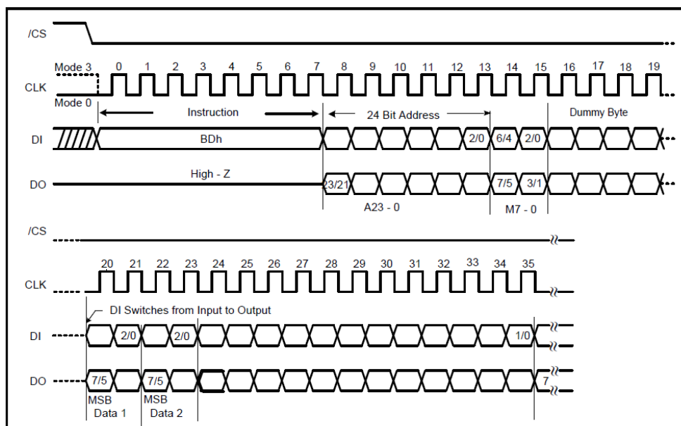
Figure18c. DTR Read Dual I/O Instruction (Previous instruction set M5-4 \neq 10, SPI Mode)
