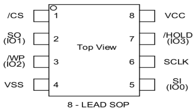
Figure 1a. 8-pin SOP 208-mil/150-mil
